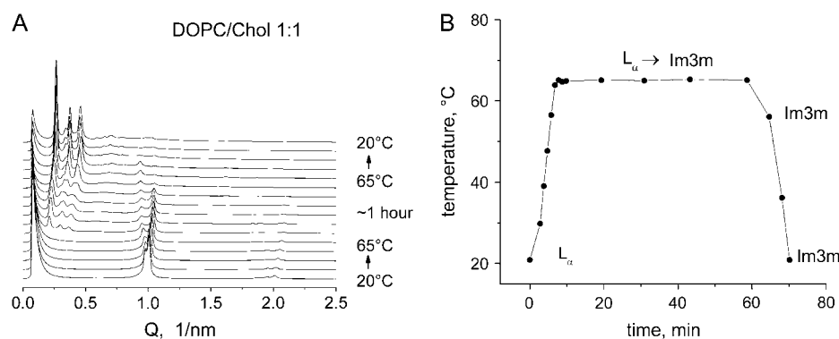
FIGURE 2 (A) Sequence of x-ray diffraction patterns showing a lamellar-to-cubic phase conversion ( L_\alpha \rightarrow Im3m ) in DOPC/Chol 1:1 mixture, 10% (w/v) in \times 10 PBS, on incubation at 65°C, followed by cooling to 20°C. (B) Temperature protocol for the L_\alpha \rightarrow Im3m conversion in A.
