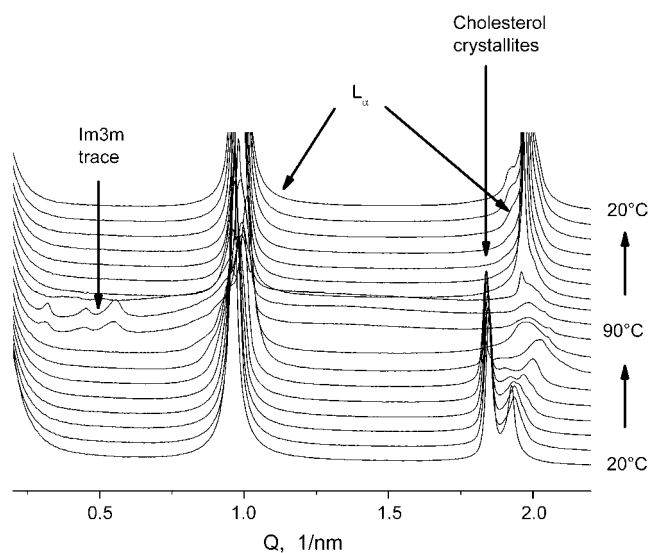
FIGURE 5 Transient cubic phase trace at high temperature in POPC/Chol 3:7 mixture, 10% (w/v) in PBS. Sequence of x-ray diffraction patterns recorded at every minute. Scan rate 10^\circ\text{C}/\text{min} .
