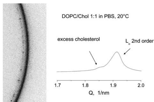
FIGURE 7 Diffraction from excess Chol crystallites in the L_{\alpha} phase of a DOPC/Chol 1:1 mixture, 10% (w/v) in PBS, 20°C. (A) Cutoff from a 2-D diffraction pattern. (B) Axially integrated 1-D pattern obtained from the 2-D pattern in A.
